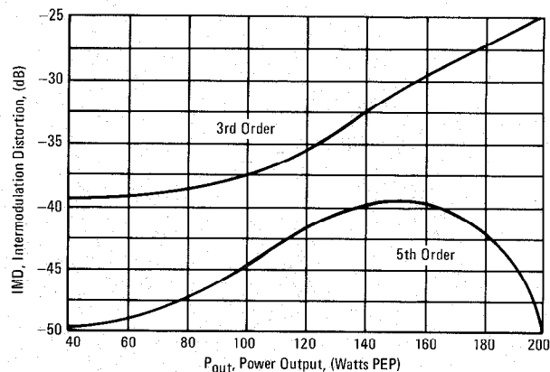
FIGURE 2—Intermodulation Distortion Versus P out , 30 MHz, 13.6 Vdc
